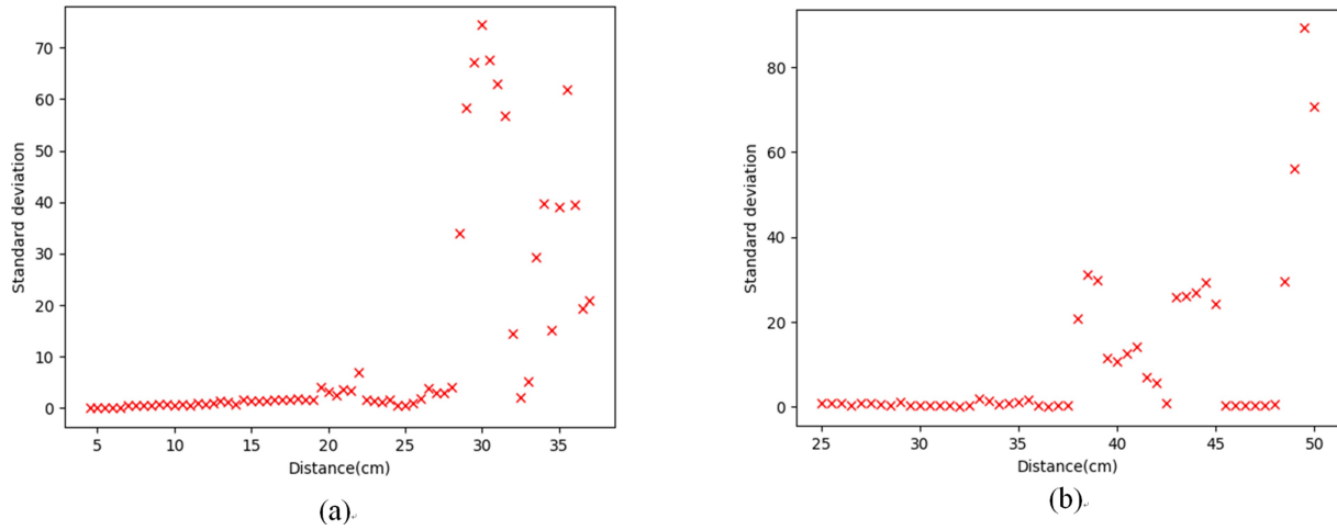
Fig. 10 Variation of the standard deviation Vs contact distance from the hinge point (a) probe length 40 cm (b) probe.
