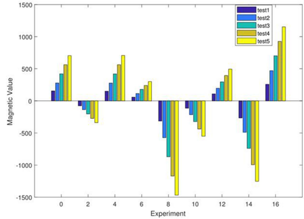
Fig. 5 The magnetic field value measured by the sensors when different currents are applied to the coil. When the current is applied to the coil, the magnetic field value is measured by the sensor. Each color represents the same current value. The five currents in the figure are 1I, 2I, 3I, 4I, and 5I. The nine sets of data in the figure are the measured values of 9 randomly selected directions from 24 directions (obtained from eight sensors).
