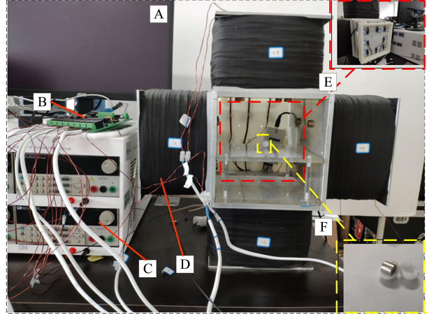
Fig. 1 The proposed driving and tracking system.
