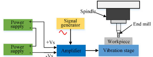
Fig. 7 Schematic diagram of the vibration stage and the machining process.
