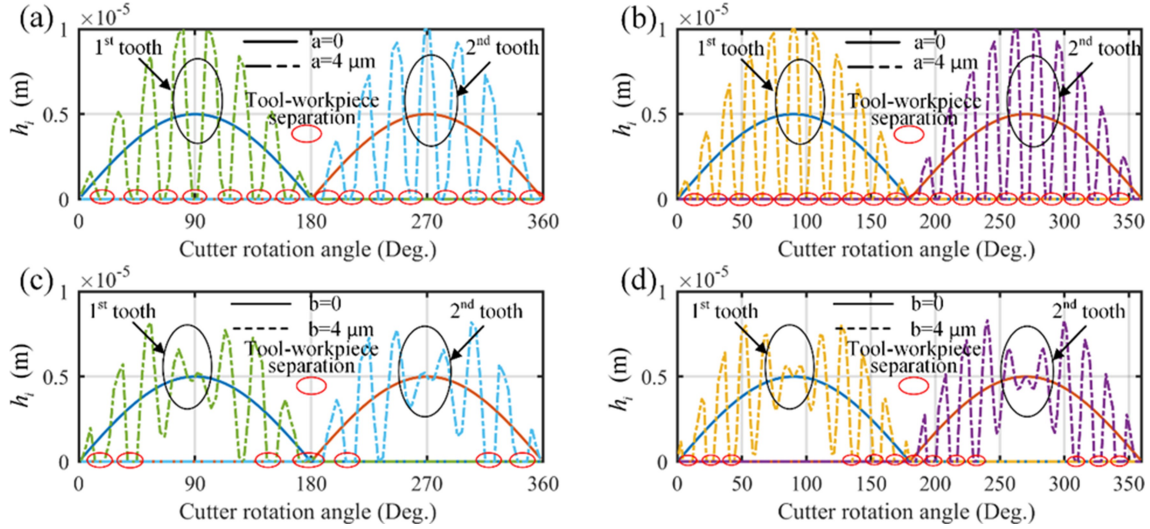
Fig. 3 Instantaneous uncut chip thickness with different vibration conditions:
