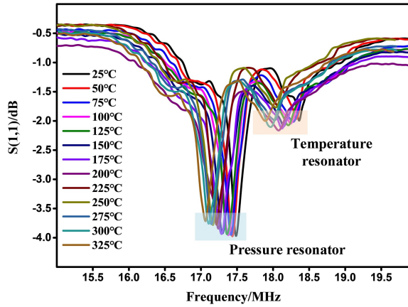
Fig. 6 Measured frequency versus S(1,1) of the sensor under ambient pressure at 25-325 °C
