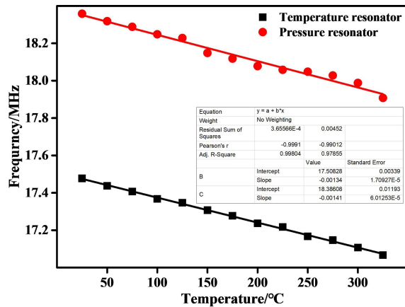
Fig. 7 Fitting curve for the pressure resonator and the temperature resonator.
