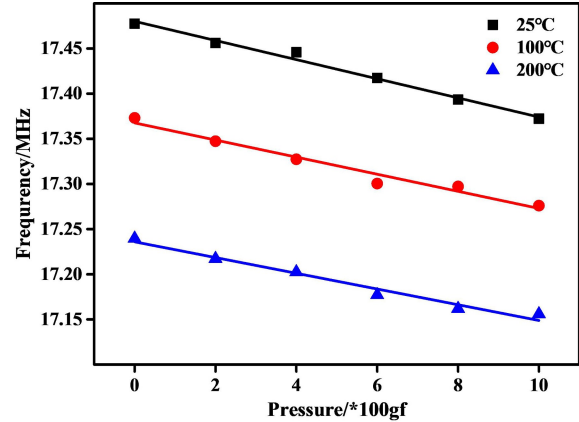
Fig. 8 Pressure measurement.
