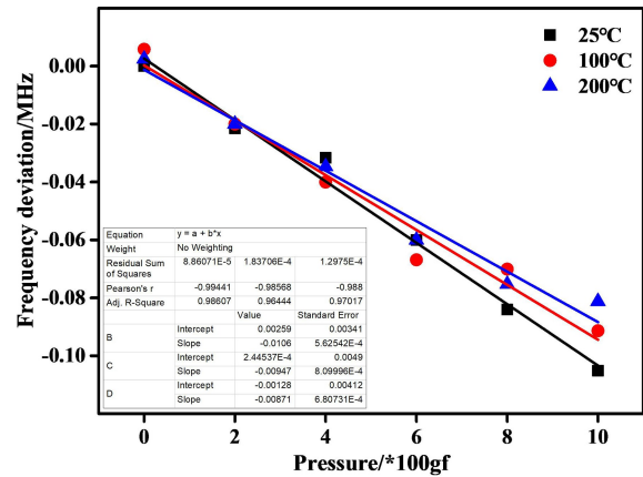
Fig. 9 Pressure sensitivity of the developed pressure resonator.
