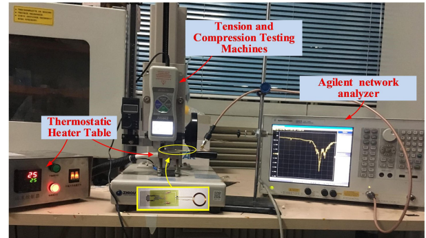
Fig. 5 Measurement equipment of the temperature-pressure SAW-based sensor.
