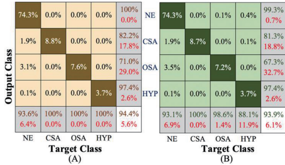
Fig. 3 Confusion matrices for SVM trained data; (A) OVO (B) OVA approach
