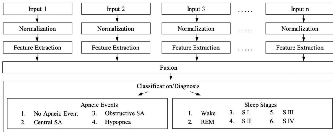
Fig. 1 Classification of the fused data from all signals.
