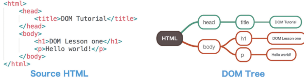
Fig. 3 source HTML and DOM tree.
