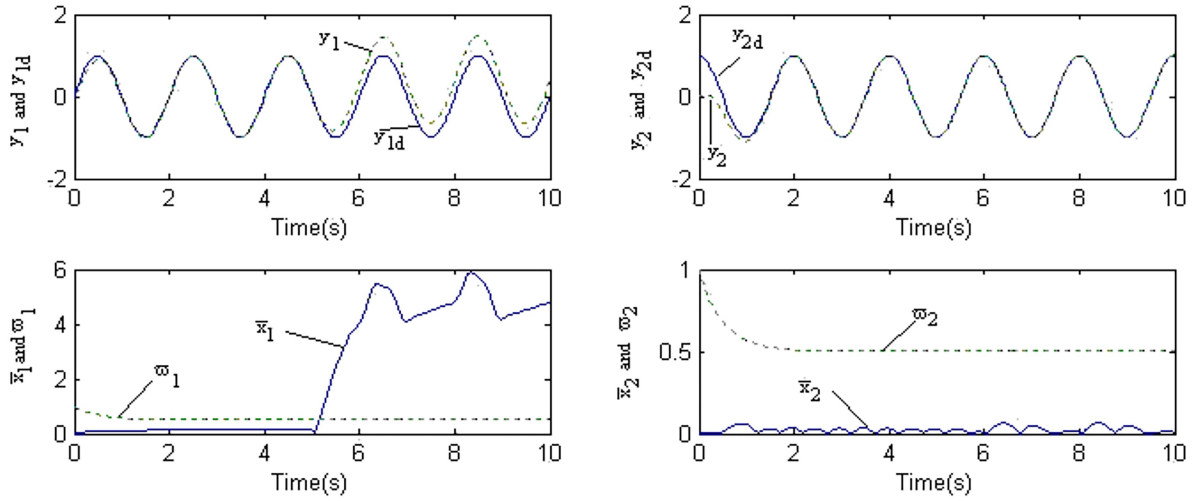
Fig. 2 Simulation results: original control without fault-tolerance (top) ; fault diagnosis (bottom)
