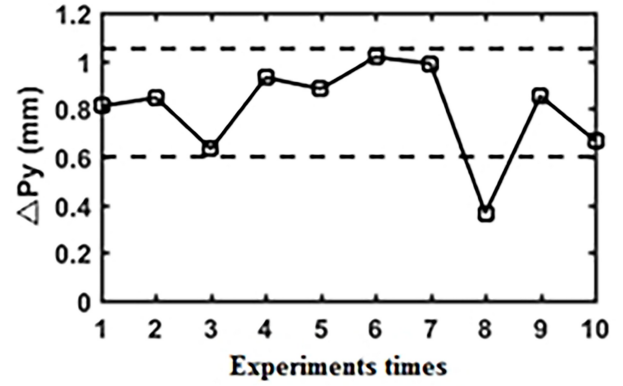
Fig. 6 The center points distribution of the target peg and hole.
