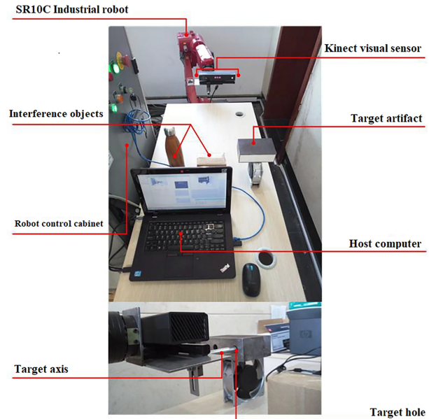
Fig. 4 The experimental platform.
