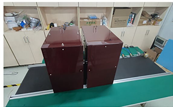
Fig. 1 (a) Schematic diagram of the sorting system. 1-conveyor, 2-LED, 3- CCD cameras, 4- structured laser, 5-photoelectric switch, 6-high pressure jet system, 7-synchronous wheel encoder; (b) A view of the real system.
