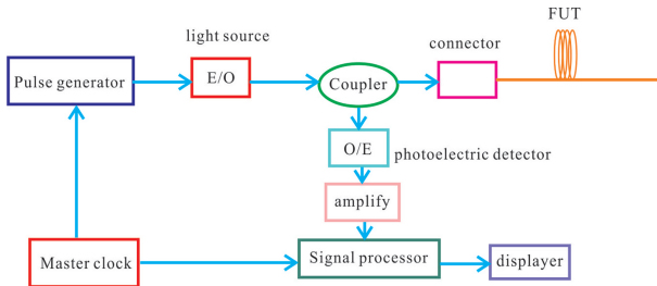
Fig. 1 Structural diagram of OTDR
