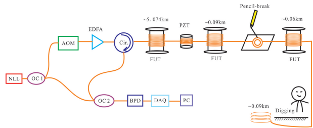
Fig. 7 Block diagram of the DAS system.
