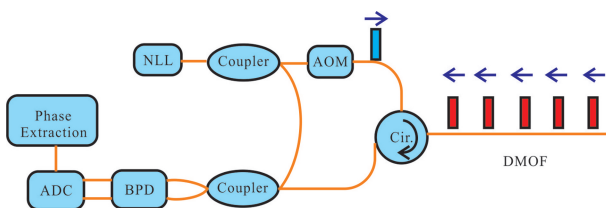
Fig. 8 Block diagram of the DAS system for borehole seismic exploration.
