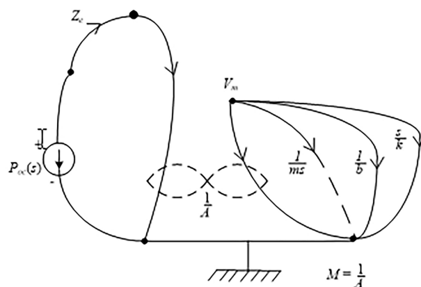
Fig. 5(d) The TF LG with the fluid domain in the Thevenin form.
