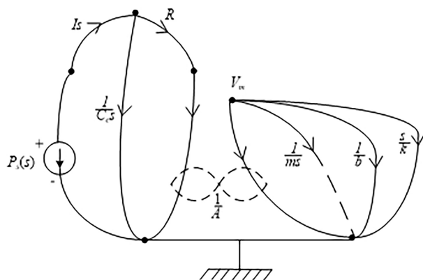
Fig. 5( c ) The Transfer-function linear graph of the fluid-mechanical system.
