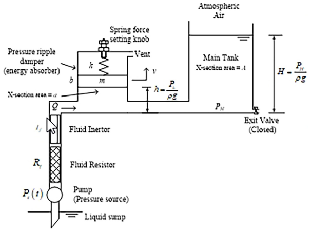
Fig. 2 A liquid pumping system.
