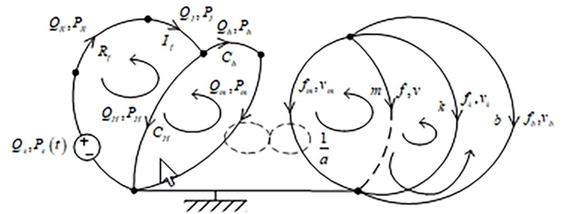
Fig. 3 Linear graph of the system.
