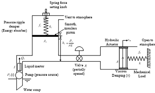
Fig. 4 Water pumping system for a hydraulic actuator.
