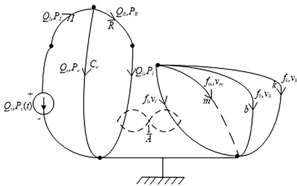
Fig. 5(b) LG of the equivalent system with independent energy storage elements.
