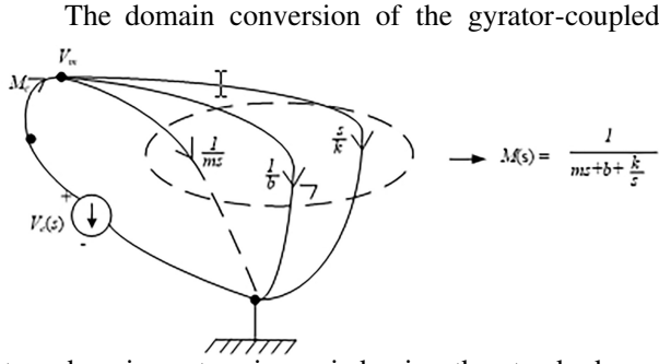
Fig. 5(e) The equivalent TF LG entirely in the mechanical domain.
