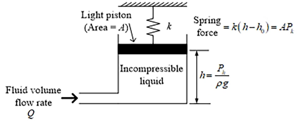
Fig. 1 Two series capacitors in a fluid-mechanical device.
