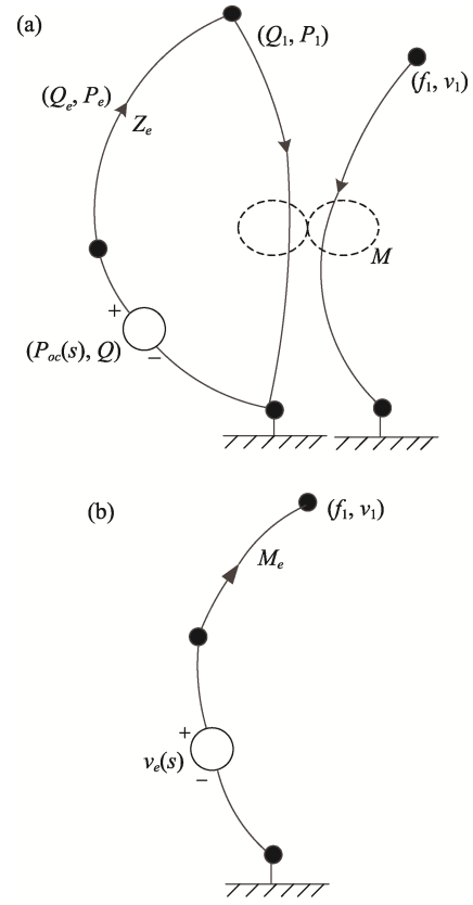
Fig.6 Gyration-coupled System. (a) Thevenin equivalent LG of the subsystem to be converted; (b) Equivalent transfer-function LG of the subsystem in the new domain
