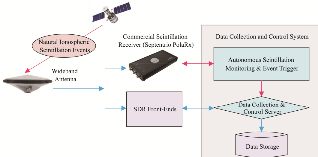
Fig.2 Data Collection System Driven by Ionospheric Scintillation
