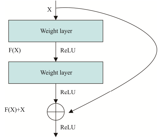
Fig.4 Residual Network
