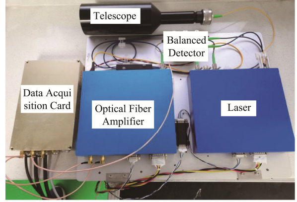
Fig.4 Physical Picture of the Experimental System
