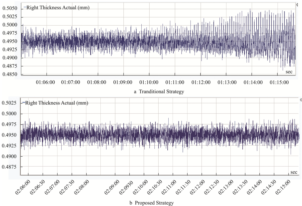
Fig.6 Product Thickness Curve
